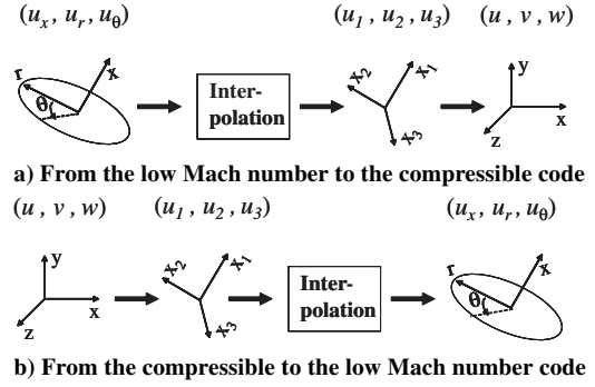
Fig. 3 Transformation of velocities between the coordinate systems of the two codes.
